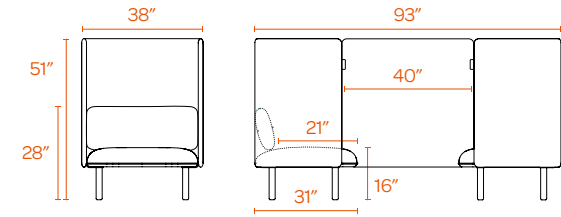
LOUNGE CHAIR BOOTH
